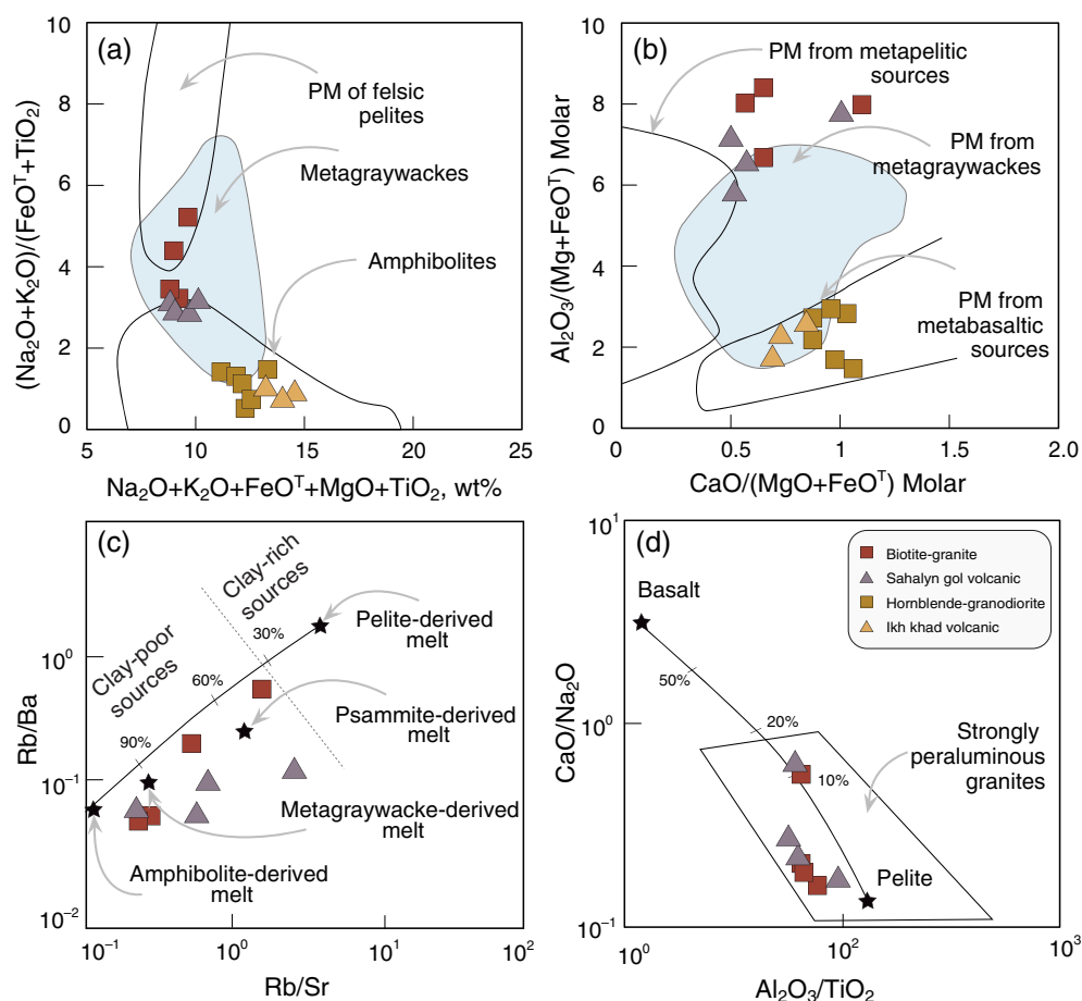
FIGURE 10 (a) (\text{Na}_2\text{O} + \text{K}_2\text{O})/(\text{FeO}^T + \text{TiO}_2) versus \text{Na}_2\text{O} + \text{K}_2\text{O} + \text{FeO}^T + \text{MgO} + \text{TiO}_2 , wt% diagram, (b) molar \text{Al}_2\text{O}_3/(\text{Mg} + \text{FeO}^T) versus molar \text{CaO}/(\text{MgO} + \text{FeO}^T) for source determination, (c) Plots of Rb/Ba versus Rb/Sr, (d) \text{CaO}/\text{Na}_2\text{O} versus \text{Al}_2\text{O}_3/\text{TiO}_2 plots for source characteristics (Patiño Douce & Harris, 1998; Patiño Douce & Johnston, 1991)
