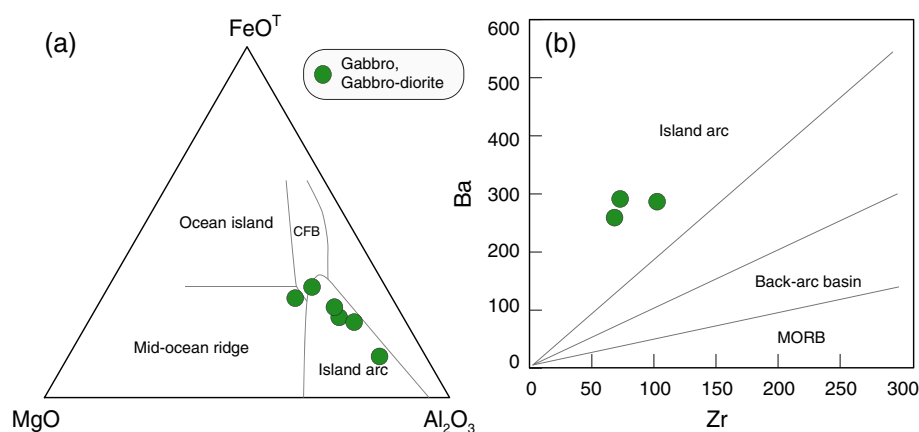
FIGURE 12 (a) \text{MgO}-\text{Al}_2\text{O}_3-\text{FeO}^T ternary diagram for tectonic discrimination of mafic rocks from the Middle Gobi Belt (Pearce et al., 1977); (b) Ba versus Zr tectonic discrimination diagram of mafic rocks from the Middle Gobi Belt (Shervais, 1982)
