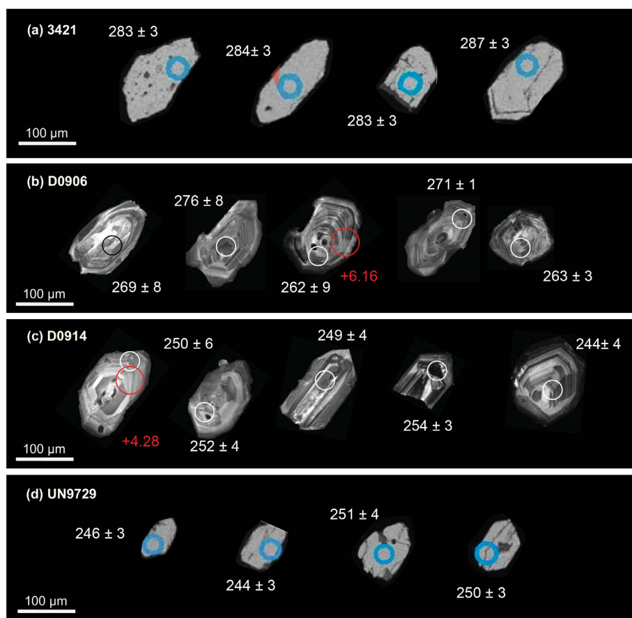
FIGURE 7 Cathodoluminescence (CL) images of representative zircon crystals from the studied samples from the Middle Gobi Belt. White circles show individual analysis spots, corresponding U–Pb ages and red circles show an individual spot of Lu–Hf isotope and their \varepsilon_{\text{Hf}}(t) values
